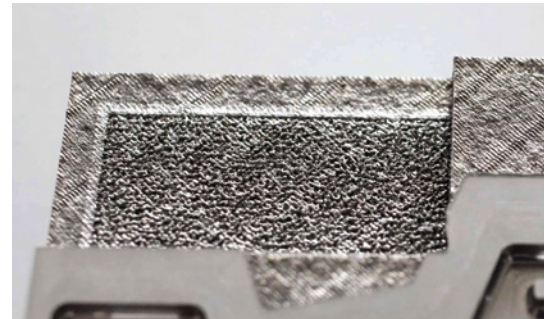
Poröse Bauweise Lumex / Hybrid Additive Manufacturing
